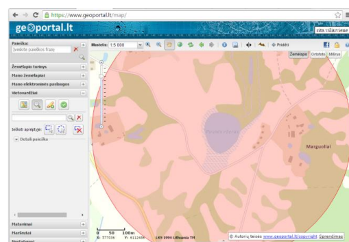
Fig. 2 Location of hydronyms near the analyzed lake.
